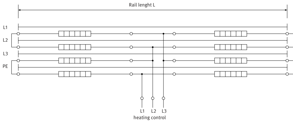
Example: Center current feed (3-conductors + PE)
