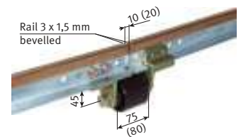
Value in brackets for 20 mm air gap
