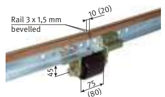
Value in brackets for 20 mm air gap
