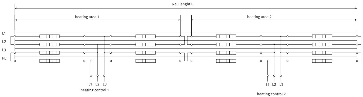
Example: Conductor de-icing with several heating sections (3-conductors + PE)
