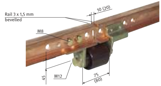
Measures in brackets for 20 mm air gap
