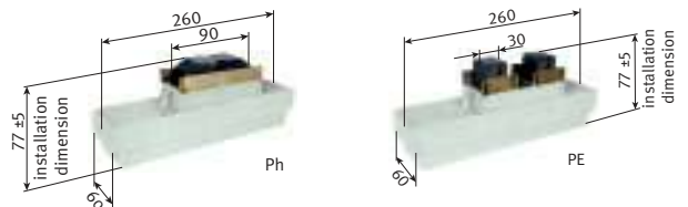
Wear height of the carbon brushes 20 mm
